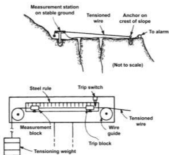
Fig. 24: Tensioned wire strain meter (Dunncliff & Green, 1993)
