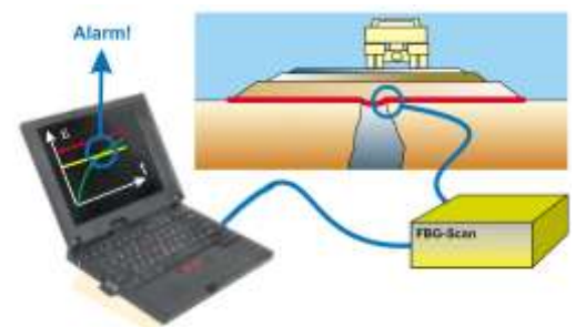
Fig. 37: Geodetect system configuration (Illustration: Polyfelt Geosynsnetics)
