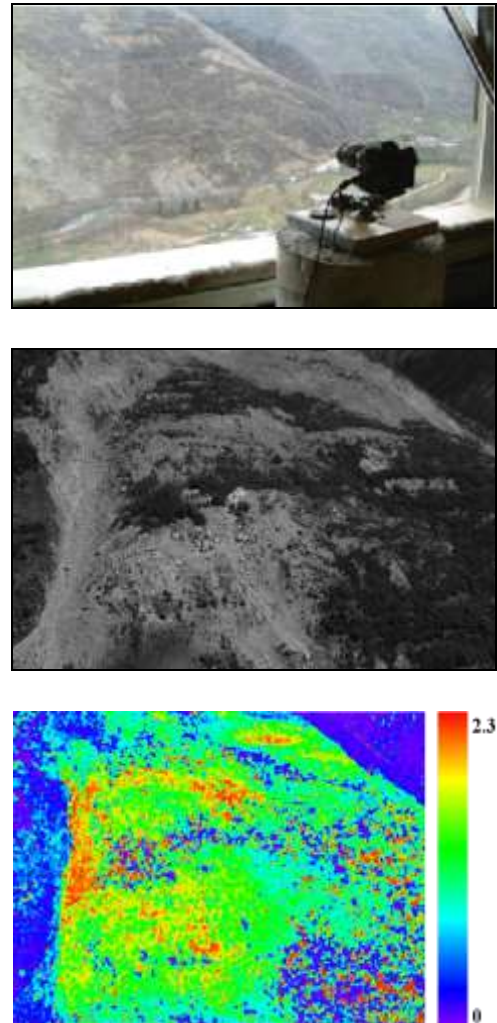
Fig. 41: Fixed camera installed in front of the “La Clapière” landslide. Photograph and displacement map (in pixels) derived from two images (Dela-court et al., 2007)
