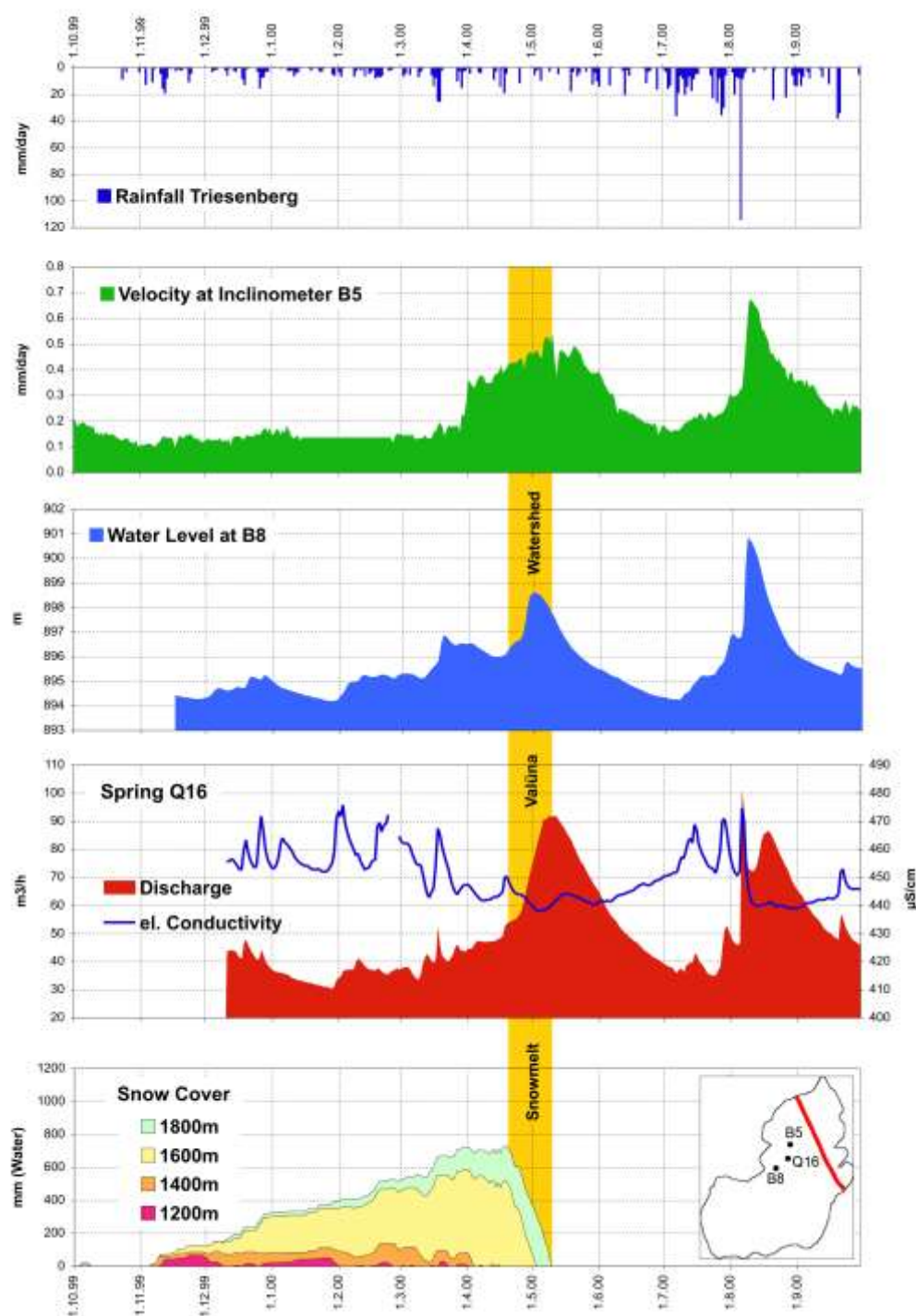
Fig. 91: Graph of the continuously collected data in the inclinometric tube B5, with the piezo-metric device B8, and of the discharge of spring Q16. The location of these observation points is depicted in the inset map.
