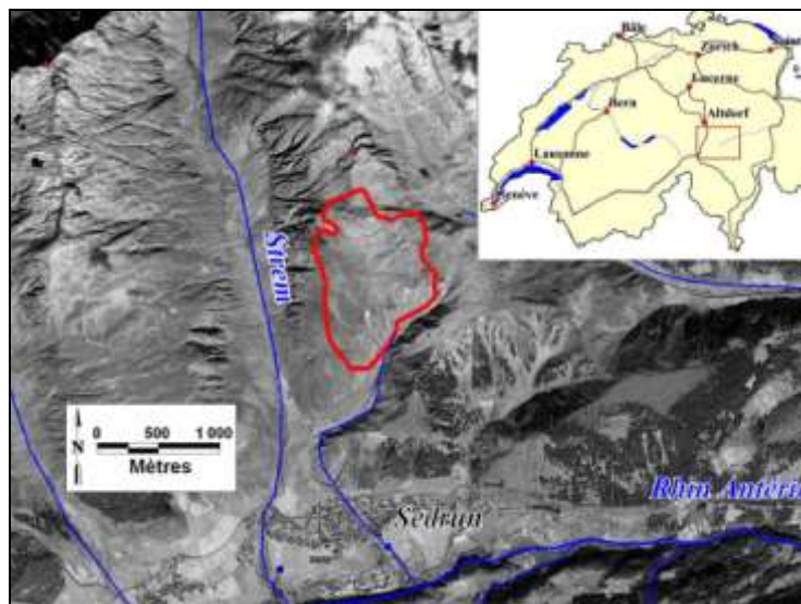
Fig. 65: Location of the Sedrun Landslide
